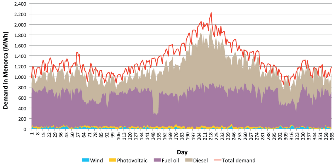
▲ Figure 5.3. Coverage of daily electricity demand in 2013. The difference between total demand and total production corresponds to the electricity exchanged via the Mallorca-Menorca submarine power cable. Source: Prepared by the authors using data from the Spanish Electricity Network.
