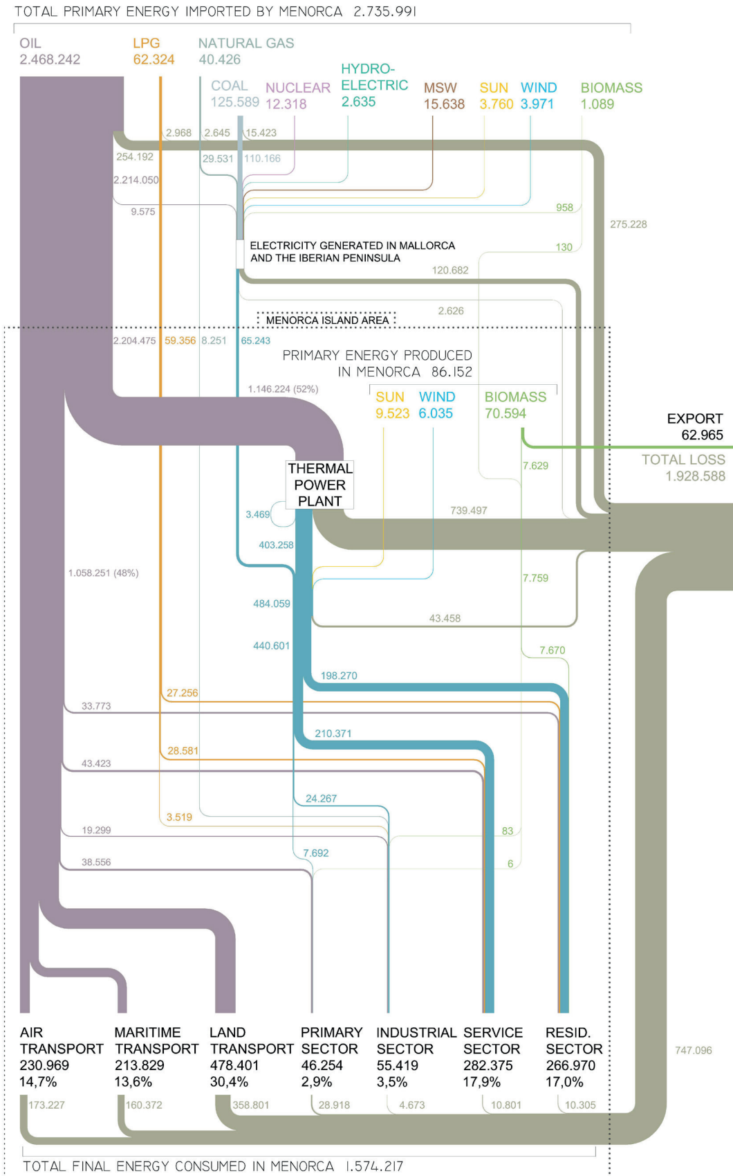
▲ Figure 4.1. Sankey diagram of Menorca's energy system, 2013. Units: MWh. Source: Prepared by the authors.
